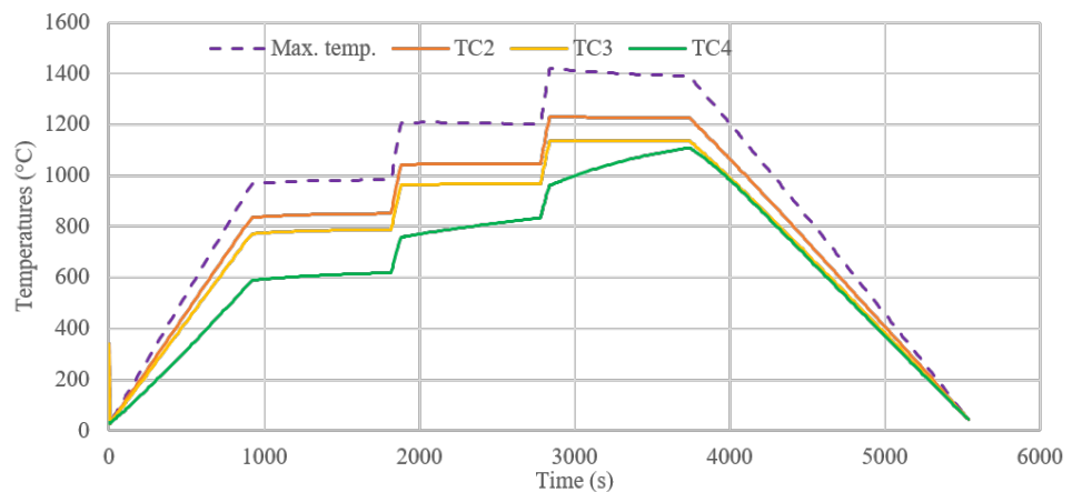
Figure 13. Full simulated thermograms of experiment #P4.
