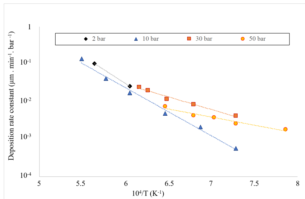
Figure 5. Arrhenius plots of the reaction rate for 4 different pressures.
