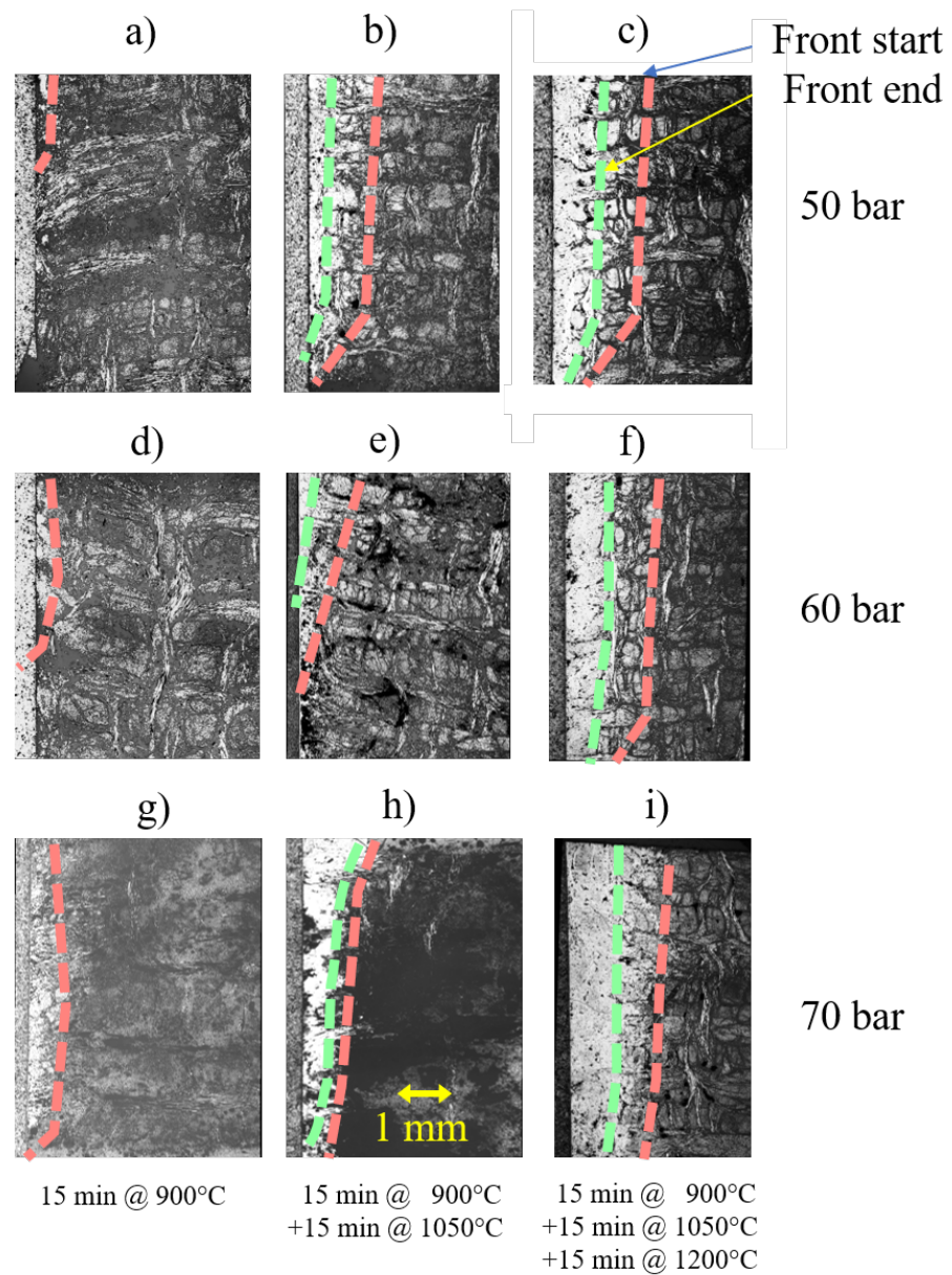
Figure 10. (a–i) Transverse micrographs of samples obtained after runs #P2 to P10, respectively. The scale bar is common to all micrographs. The approximate locations of the front starts and ends are indicated by red and green dashed lines, respectively.
