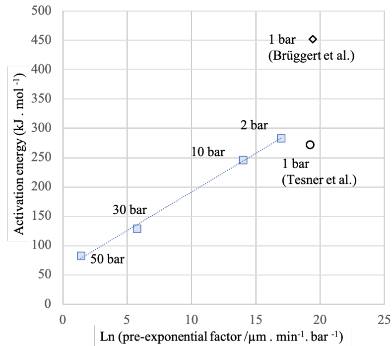
Figure 6. Pre-exponential factor—activation energy diagram for methane deposition at various pressures and following various authors. The dotted line is a guide for the eye to the data from this study.
