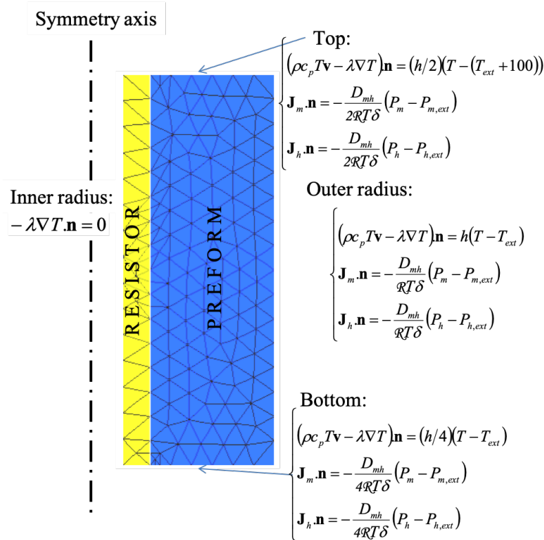
Figure 11. Geometry and boundary conditions for the model.
