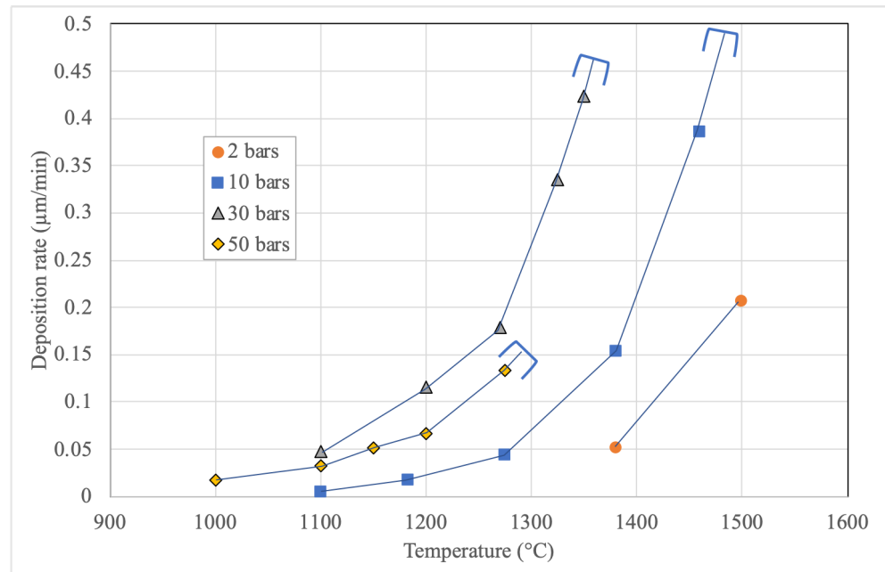
Figure 3. Deposition rate on the single filament as a function of temperature and for different methane pressures. The start of the observed homogeneous nucleation is indicated by the brackets ending the tendency curves for 10, 30, and 50 bars.
