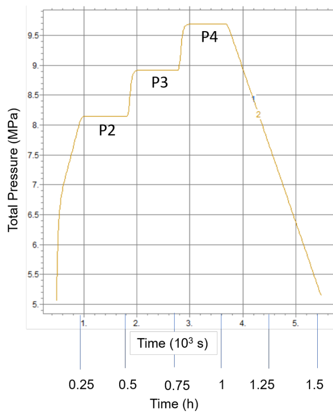
Figure 14. Simulated evolution of the total pressure for experiments #P2 to P4.
