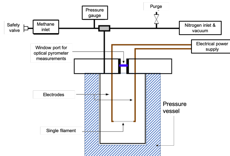
Figure 2. Scheme of the setup for the determination of reaction kinetics on a single filament.
