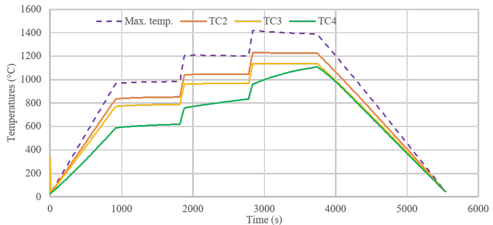
Figure 13. Full simulated thermograms of experiment #P4.
