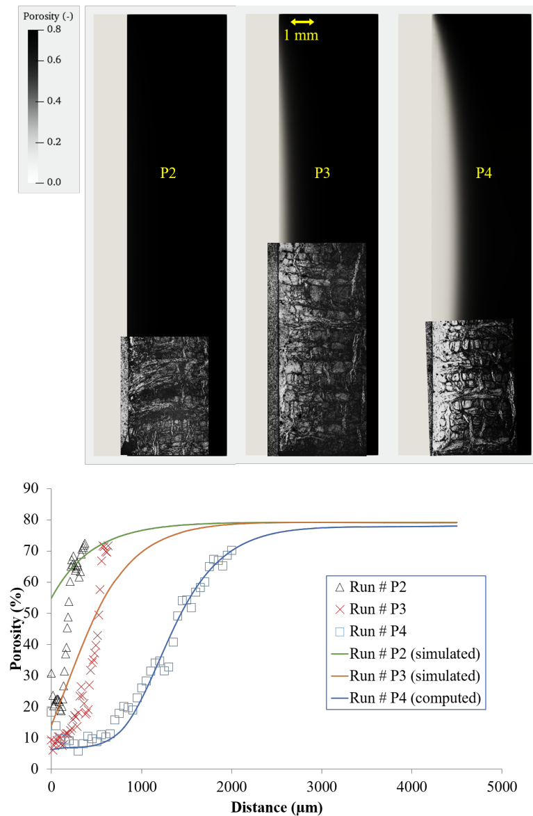
Figure 16. Simulated infiltration runs #P2–4: porosity profiles: (top) 2D computed profiles compared to micrographs on the same scale; (bottom) comparison of the porosity profiles obtained at the half-height of the preform.
