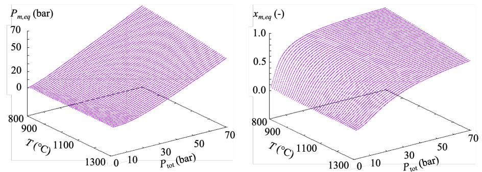
Figure 4. Equilibrium partial pressure of methane (left) and equilibrium mole fraction of methane (right) for the deposition reaction (1) as a function of temperature and total pressure.
