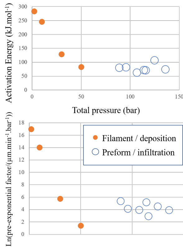
Figure 15. Kinetic parameters vs. total pressure in CVD and CVI experiments. The size of the symbols indicates the experimental uncertainty.
