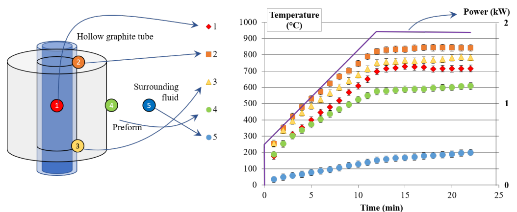
Figure 7. Thermal study: (left) position of the thermocouples; (right) thermal history.
