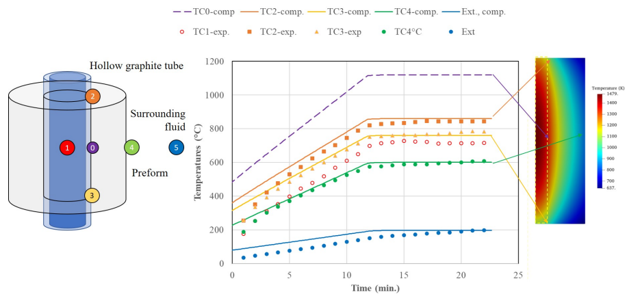
Figure 12. Computation of the thermal histories of selected points of the setup: (left) position of the sampled points; (right) thermal history of these points compared to experimental ones.
