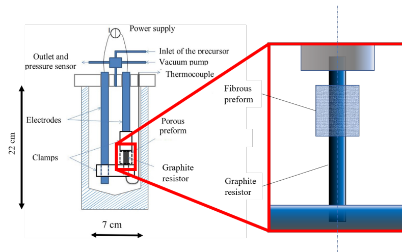
Figure 1. Scheme of the setup, with the porous preform settled around the graphite resistor.
