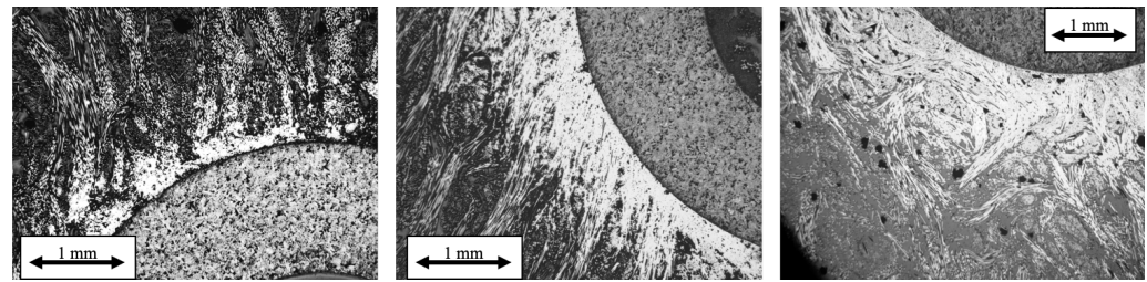
Figure 8. Micrographs of the cross-section for 3 successive infiltrations #P2, P3, and P4, from left to right.
