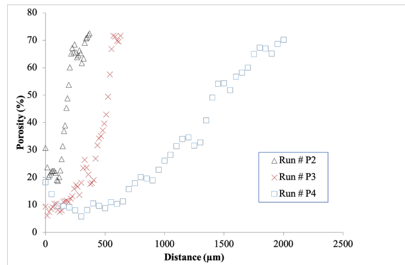
Figure 9. Porosity profiles for 3 successive infiltrations #P2, P3, and P4.
