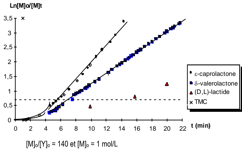
Figure 1 : Variation of \text{Ln}[M]_0/[M]_t with time, for different cyclic monomers polymerized with [\text{Y}(\text{OCH}_2\text{CH}_2\text{O}i\text{Pr})_3]_2 in dichloromethane solution at room temperature.
