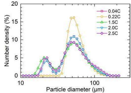
Fig. 2. Particle size distributions of raw powders used in this study.
