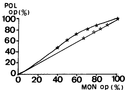
Fig. 1. Optical purities (o.p.) of prepared poly lactides vs reacting monomers. Initiators: ★ \text{SALENAlOCH}_3 (Ref. 32) ☆ Sn octoate (Ref 25) (—) theoretical line for statistical enantiomeric distribution.
