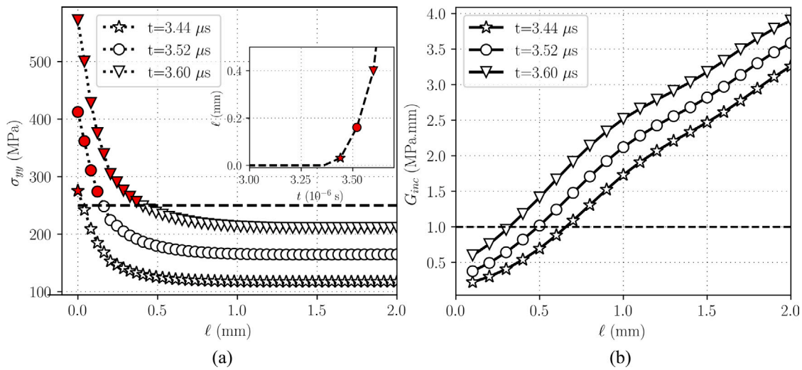
Fig. 22. (a) Stress variation along the V-notch bisector prior to crack initiation and (b) incremental energy release rate as a function of the crack length.
