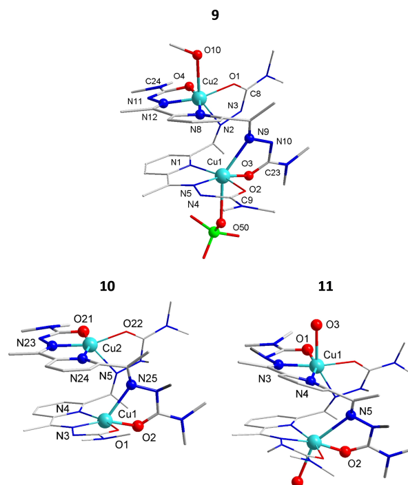
Figure 5. Crystal structures of the molecular complexes in [\{\text{CuH}_2\text{L}^{\text{NMe}_2}\}_2(\text{ClO}_4)(\text{MeOH})] \cdot (\text{ClO}_4)_3 \cdot 1\text{H}_2\text{O} \cdot 1.75 \text{ MeOH} , 9 , [\text{CuHL}^{\text{NMe}_2}]_2 \cdot (\text{ClO}_4)_2 \cdot \text{H}_2\text{O} , 10 , and [\text{CuH}_2\text{L}^{\text{NMe}_2}(\text{H}_2\text{O})]_2 \cdot (\text{ClO}_4)_4 \cdot 5\text{H}_2\text{O} , 11 . The anions, lattice solvent molecule, and H-atoms are not shown except the H atoms of the N-hydrazone moieties.
