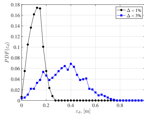
Fig. 5. Probability Density Function of the error in the distance computation, [27].
