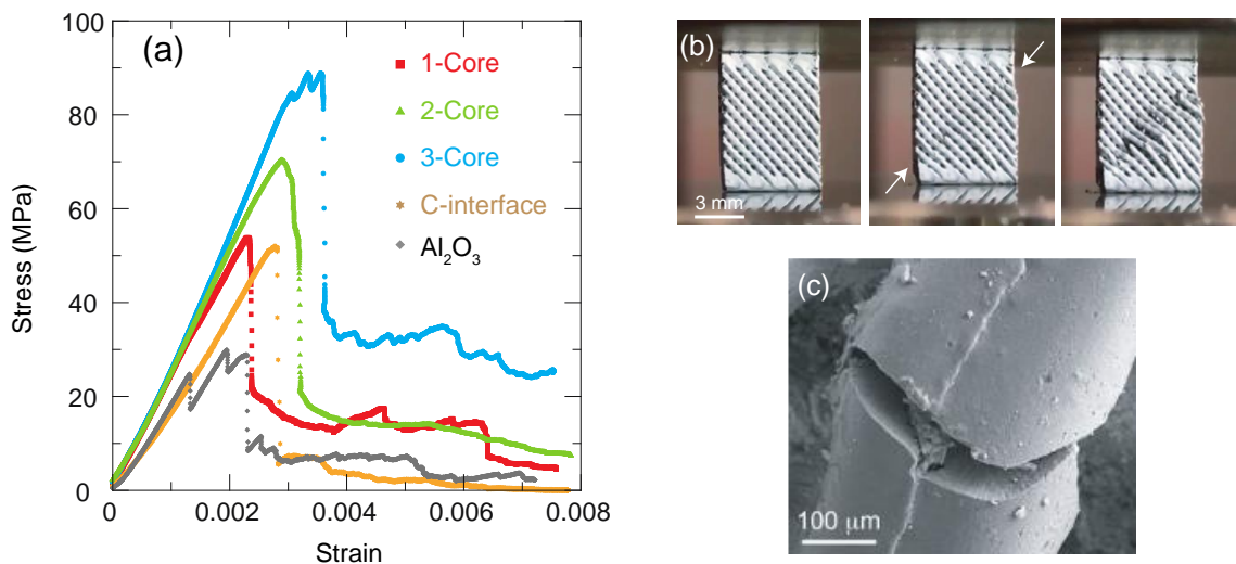
Figure 6. (a) Stress displacement curves from compression tests performed on the woodpile structures. The ceramic grids break in the gradual manner observed in other ceramic woodpile structures with drops corresponding to individual strut failures. In the structures with steel cores the struts fail by buckling and they retain strength even after relatively large displacements (b) Stills taken during the compression of a 3-core wood pile structure clearly show buckling of the struts along a kink band (white arrows) (c) SEM micrograph of a fractured filament (3-core) in a woodpile structure. The ceramic shell has broken but the steel fibres are still able to maintain it together.
