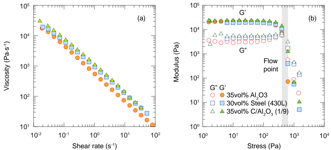
Figure 2. Rheology of the pastes used in the printing process. (a) Variation of the viscosity with shear rate. The viscosity of the pastes and their shear thinning coefficients match ( n \sim 0.1 ). (b) The viscoelastic response of the pastes also matches.
