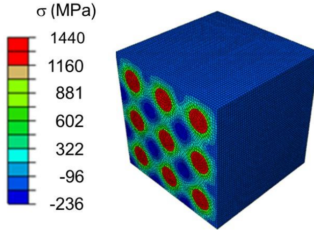
Figure 11. Finite element calculations of thermal stresses parallel to the steel fibers after cooling from 1400 °C in a composite fabricated with a 1-core filament. A compressive stress develops in the alumina matrix.
