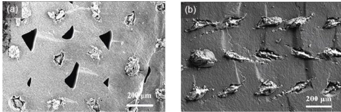
Figure 10. Scanning electron micrographs of the fracture surfaces of printed bars (1-core filaments) (a) without CIP after printing and (b) with CIP. Isostatic pressing helps to close pores trapped between the printed lines and is used for all the bars tested in this work.
