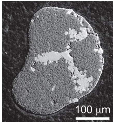
Figure 9. Cross sections of sintered filaments with 3 cores. In this system the metallic cores are highly distorted during extrusion.
