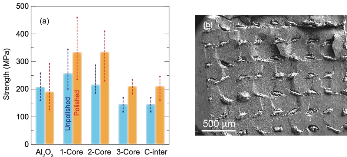
Figure 7. (a) Bending strengths of polished and unpolished bars. The inclusion of fibers increases the strength but the porous fiber-matrix interlayer decreases it. Polishing the tensile surface has an effect on the strength of the fiber-reinforced materials suggesting the importance of surface flaws. (b) Fracture surface of a 1-core bar after a bending test. Plastic deformation of the steel fibers is visible.
