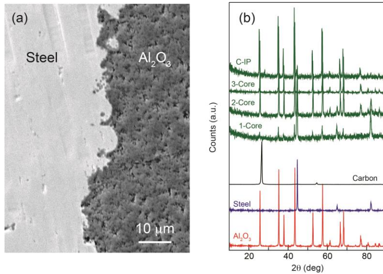
Figure 3. (a) Scanning electron micrograph showing the interface between steel and alumina after sintering. (b) X-Ray analysis of the starting powders and sintered samples. There are no additional phases after sintering and the C peaks are not visible in the samples prepared with the carbon interphase.
