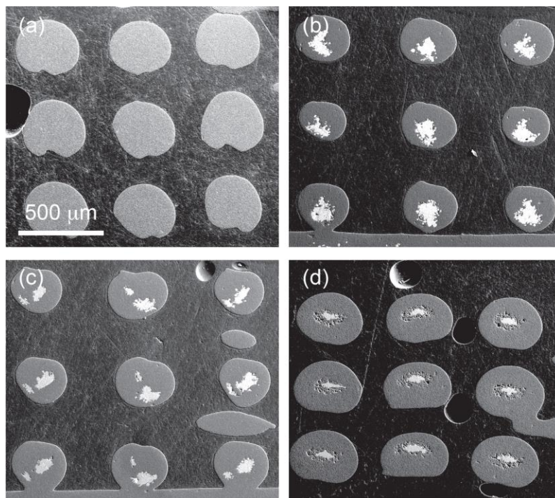
Figure 4. Polished cross sections of a sintered woodpile structure fabricated using: (a) alumina filaments; (b) 1-core, (c) 2-core and (d) 1-core with a porous interlayer (generated using a C- \text{Al}_2\text{O}_3 ink, 10/90 in vol) filaments. The steel is visible as the brighter phase in the filaments.
