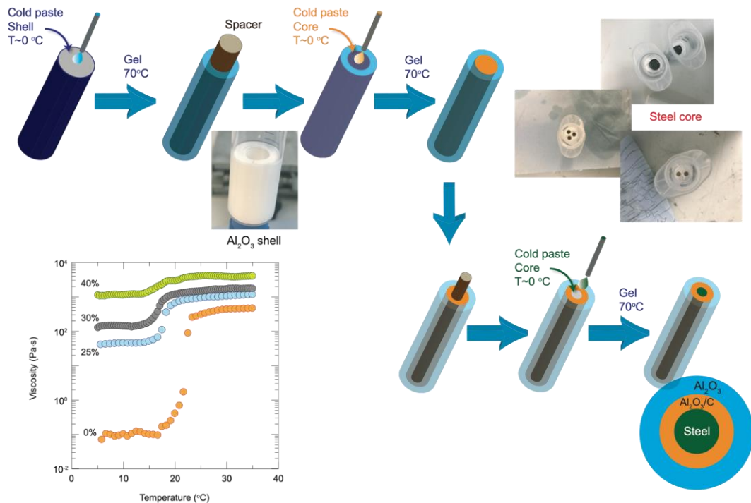
Figure 1. Process of preparing printing cartridges with core-shell structure using thermally reversible hydrogels. The graph shows the variation of viscosity with temperature for gels with different Al 2 O 3 contents (in vol%). The solid content does not have a measurable effect on the liquid-gel transition that takes place at around 18°C allowing printing at room temperature. By playing with the temperature and a set of spacers it is possible to create cartridges with a core shell structure including one to three cores. In order to engineer the interphase between the core and the shell we use a series of spacers of decreasing diameter.
