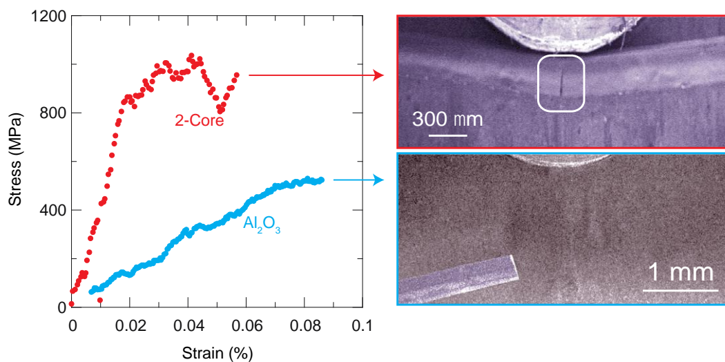
Figure 5. Bending of single filaments. Alumina filaments are brittle. The addition of the steel cores increases the bending strengths and prevent brittle filament failure.
