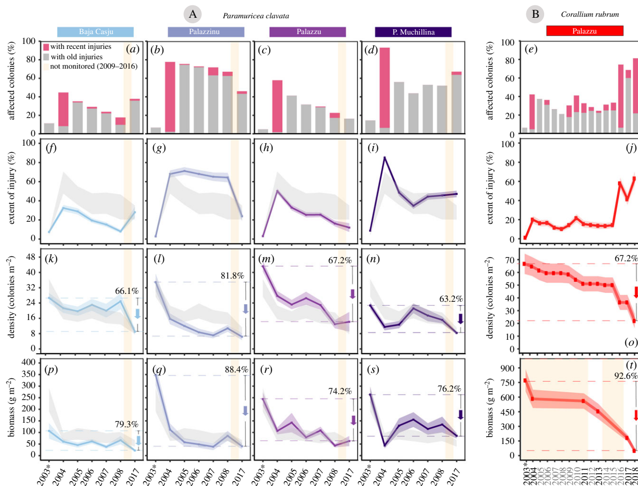
Figure 2. Temporal trends in the percentage (%) of affected colonies (a–e), percentage of extent of injury \pm s.e. (f–j), density (number of colonies per \text{m}^2 \pm s.e.) (k–o) and biomass (g per \text{m}^2 \pm s.e.) (p–t) for the monitored octocoral populations. The cumulated relative density (or biomass) loss is shown at the right side of each plot. The light grey background polygons shown in (f–j, k–n, p–s) represent the average values \pm s.e. of the four populations of P. clavata . (Online version in colour.)
