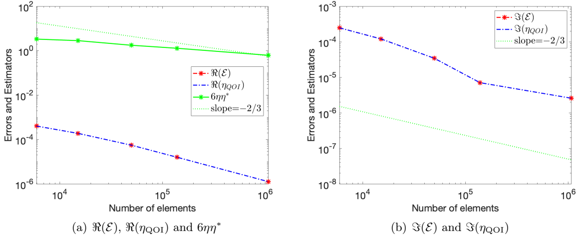
Figure 13: Error and Estimator, global refinement, \mathbf{q} given by (76).
