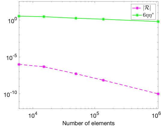
Figure 14: |\mathcal{R}| and 6\eta\eta^* , global refinement, \mathbf{q} given by (76).
