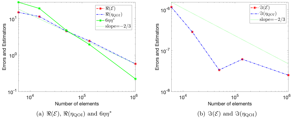
Figure 3: Error and Estimator, global refinement, \mathbf{q} = \mathbf{H}_s .
