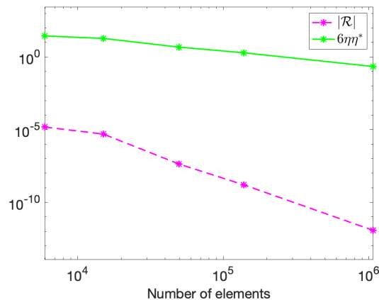
Figure 4: |\mathcal{R}| and 6\eta\eta^* , global refinement, \mathbf{q} = \mathbf{H}_s .
