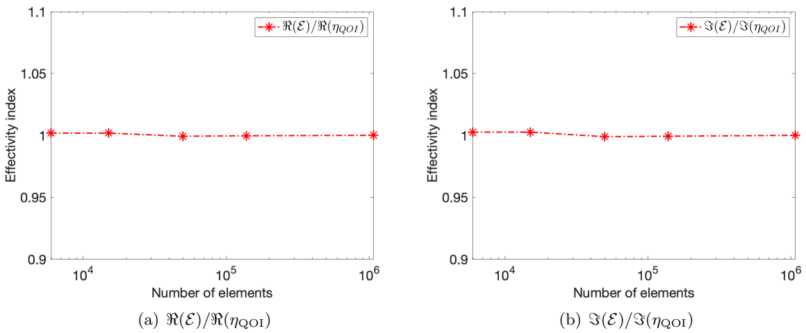
Figure 15: Ratios of error over estimator, real and imaginary parts, global refinement, \mathbf{q} given by (76).
