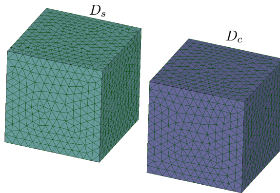
Figure 2: Mesh 4, global refinement, 138 404 elements : 9 826 elements in D_s , 9 428 elements in D_c and 119 150 elements in D \setminus (D_s \cup D_c) .
