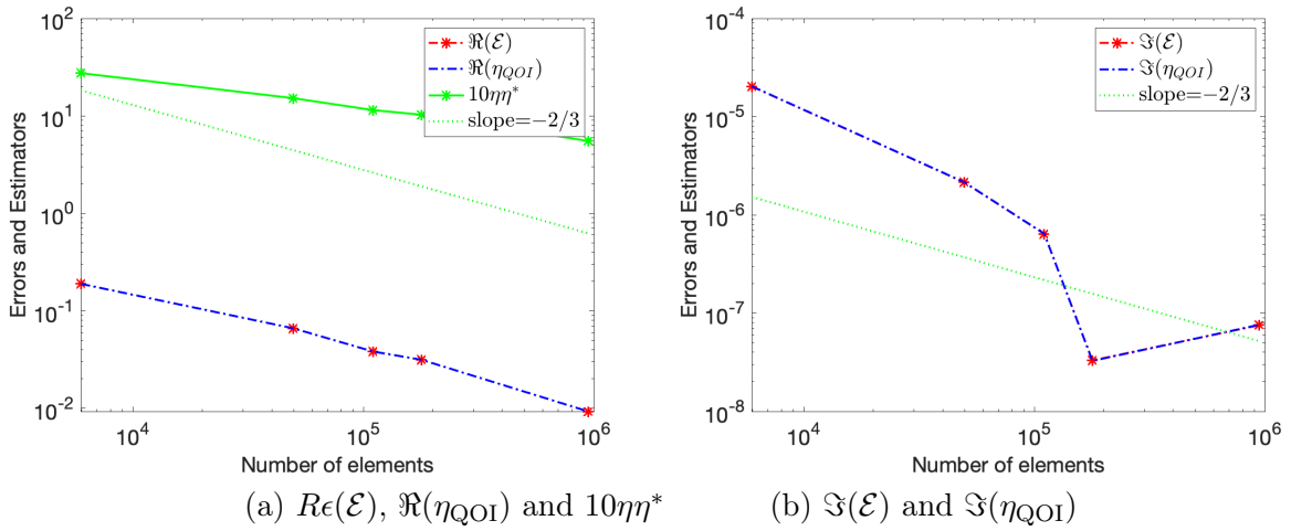
Figure 9: Error and Estimator, global refinement, \mathbf{q} given by (72).
