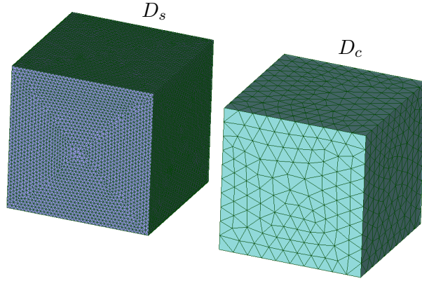
Figure 6: Mesh 3, local refinement : 243 232 elements in D_s , 5 794 elements in D_c and 103 136 elements in D \setminus (D_s \cup D_c) .
