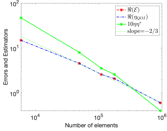
(a) \Re(\mathcal{E}) , \Re(\eta_{QOI}) and 10\eta^*
