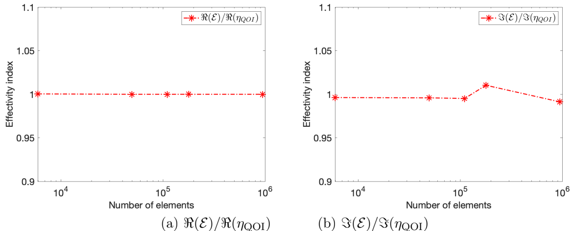
Figure 10: Ratios of error over estimator, real and imaginary parts, global refinement, \mathbf{q} given by (72).
