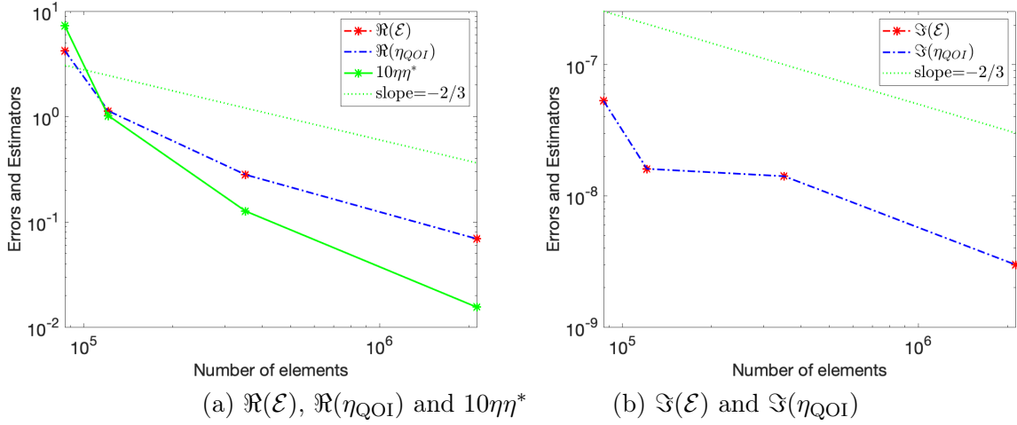
Figure 7: Error and Estimator, local refinement, \mathbf{q} = \mathbf{H}_s .
