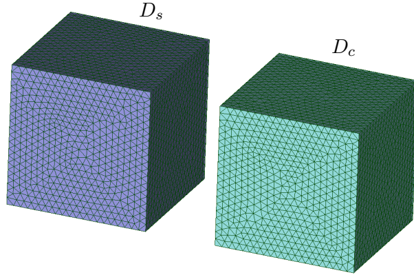
Figure 2: Mesh 4, global refinement : 12 482 elements in D_s , 12 974 elements in D_c and 153 178 elements in D \setminus (D_s \cup D_c) .
