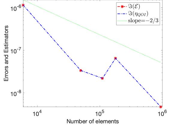
(b) \Im(\mathcal{E}) and \Im(\eta_{QOI})
