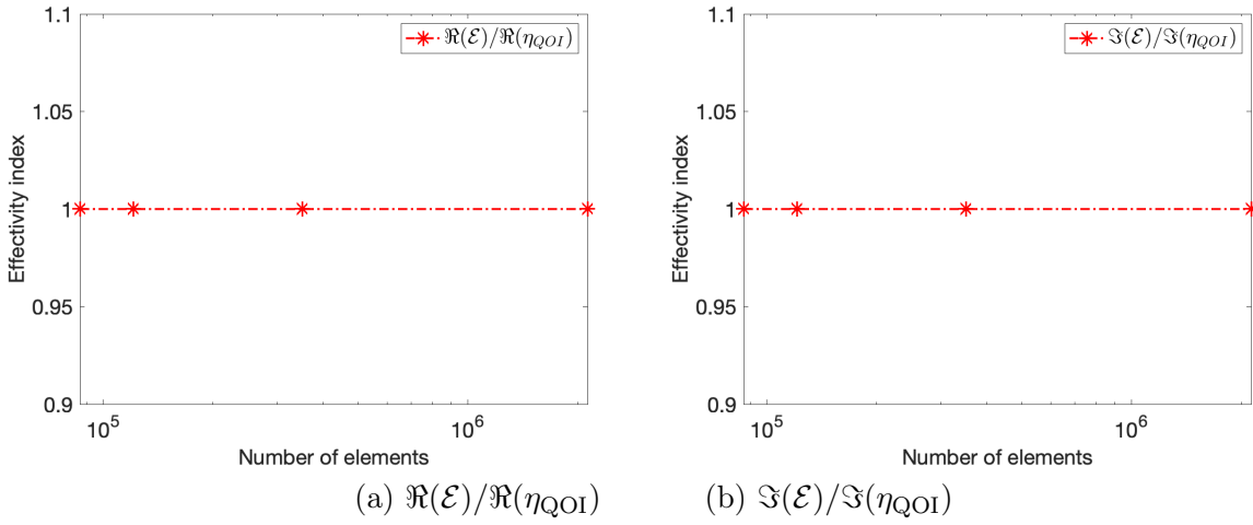
Figure 8: Ratios of error over estimator, real and imaginary parts, local refinement, \mathbf{q} = \mathbf{H}_s .
