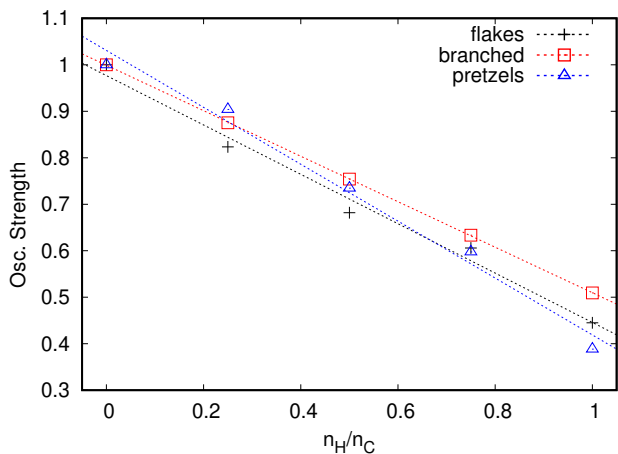
Fig. 7: Oscillator strength ratio in the [2-9 eV] region between C_{24}H_n ( n=6,12,18,24 ) and C_{24} for the flakes (black crosses), branched (red squares), and pretzels (blue triangles) families. The data points were fitted by a linear law (see Appendix B).
