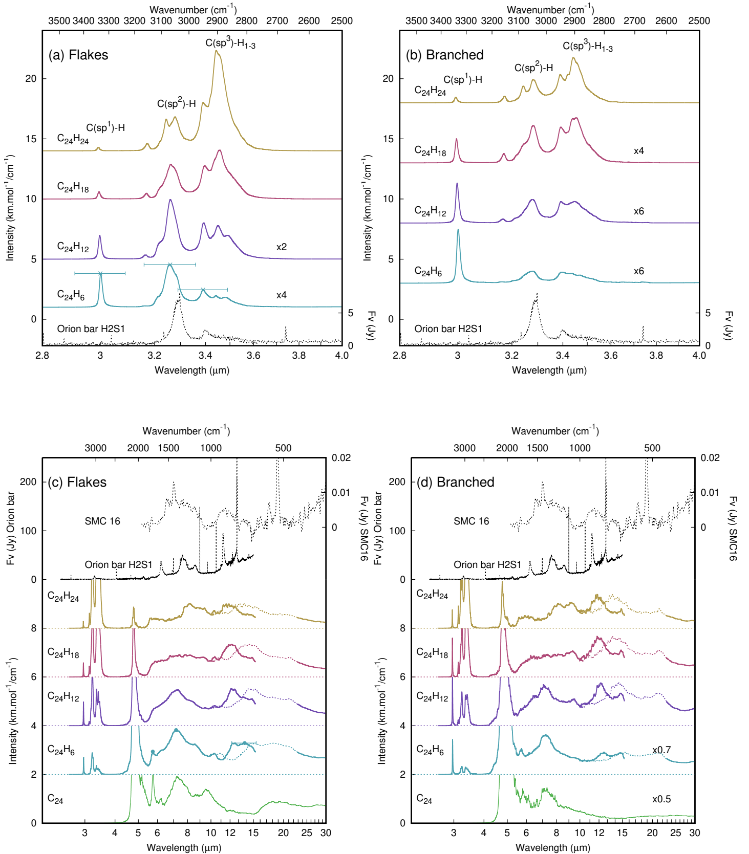
Fig. 2: Infrared spectra for the flakes and branched families and comparison with astronomical spectra. Panels (a) and (b) show a zoom into the [2.8 - 4 \mu\text{m}] region. Panels (c) and (d) show the features represented with dashed lines in the [10.2 - 22.7 \mu\text{m}] region rescaled using the appropriate factors for C-H bend (see main text and Appendix A). The final shifted band in the [10.0 - 15.3 \mu\text{m}] domain is represented in plain lines. The emission spectra from the Orion bar H2S1 (Van Dienenhoven et al. 2004) and from the SMP SMC 16 planetary nebula (García-Hernández et al. 2010) are added for comparison. Error bars are reported in panels (a) and (c) for the most intense bands of the IR spectrum of \text{C}_24\text{H}_6 flakes only, but can be applied to similar modes for all stoichiometries and families. Article number, page 5 of 16
