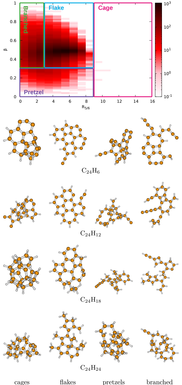
Fig. 1: Adapted from Pla et al. (2021). Two-dimensional distribution of the isomer population for C_{24}H_{12} as a function of R_{5/6} and \beta (top) and examples of isomers of C_{24}H_n for the four families (bottom).
