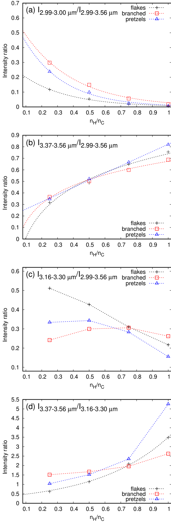
Fig. 4: Intensity ratios I_{2.99-3.00\mu\text{m}}/I_{2.99-3.56\mu\text{m}} (a), I_{3.37-3.56\mu\text{m}}/I_{2.99-3.56\mu\text{m}} (b), I_{3.16-3.30\mu\text{m}}/I_{2.99-3.56\mu\text{m}} (c), and I_{3.37-3.56\mu\text{m}}/I_{3.16-3.30\mu\text{m}} (d) as a function of the n_H/n_C fraction for the flakes family (black crosses), branched family (red squares), and pretzels family (blue triangles). The dashed lines either result from the analytical data fitting (when starting below x=0.25 ; see Table B1 in Appendix B for the coefficients) or were drawn to guide the eye.
