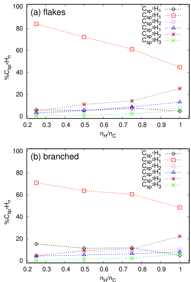
Fig. 3: Evolution of the C(sp^x)H_n ( x=1\text{-}3, n=1\text{-}3 ) fraction as a function of n_H/n_C for the flakes (a) and branched (b) families
