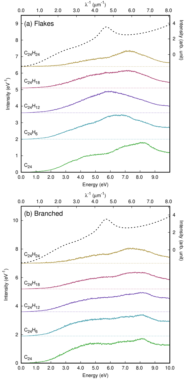
Fig. 6: TD-DFTB optical spectra of C_{24}H_n ( n=0, 6, 12, 18, 24 ) for the flakes (a) and branched (b) families. The average Galactic extinction curve adapted from Fitzpatrick & Massa (2007) is reported in dashed lines.
