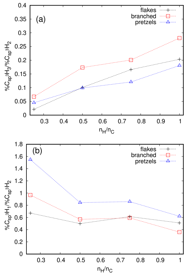
Fig. 8: Evolution of the C(sp^3)H_3/C(sp^3)H_2 (a) and C(sp^3)H_1/C(sp^3)H_2 (b) fraction as a function of n_H/n_C for the flakes, branched, and pretzels families
