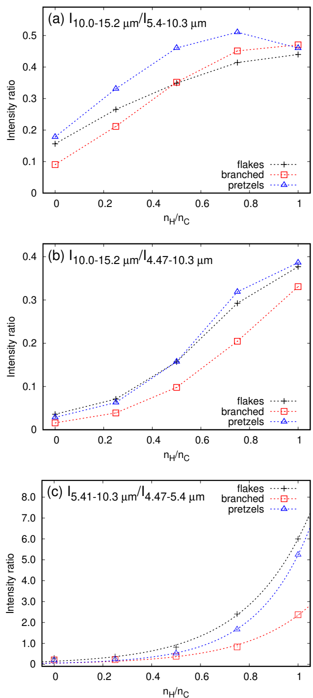
Fig. 5: Intensity ratios I_{10.0-15.2\mu\text{m}}/I_{5.4-10.3\mu\text{m}} (a), I_{10.0-15.2\mu\text{m}}/I_{4.47-10.3\mu\text{m}} (b), and I_{5.41-10.3\mu\text{m}}/I_{4.47-5.4\mu\text{m}} (c) as a function of the n_H/n_C fraction for the flakes family (black crosses), branched family (red squares), and pretzels family (blue triangles). The dashed lines in plots (a) and (b) were drawn to guide the eye, whereas in plot (c), these lines show the exponential fitting of the data (see Appendix B for the details of the fit).
