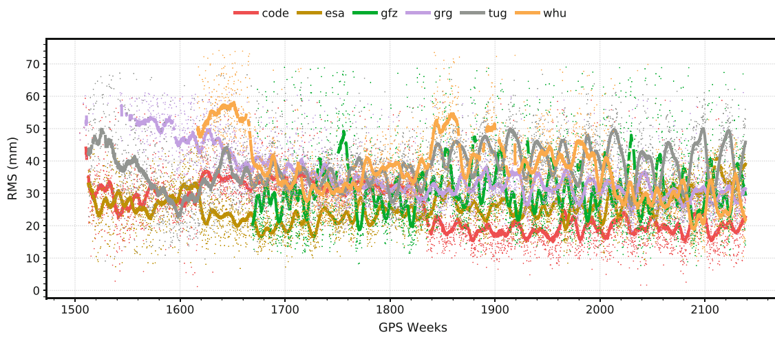
(b) GLONASS
