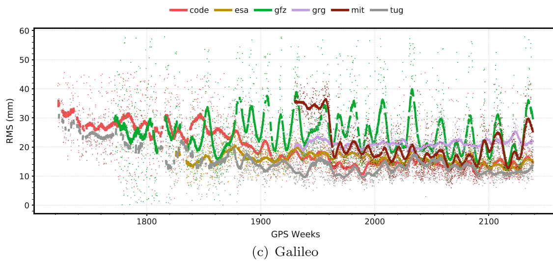
Fig. 1 3D-RMS difference of individual AC orbit solutions w.r.t the combined solution. Please note that the y-axis scales are different for each figure. (a) GPS. (b) GLONASS. (c) Galileo
