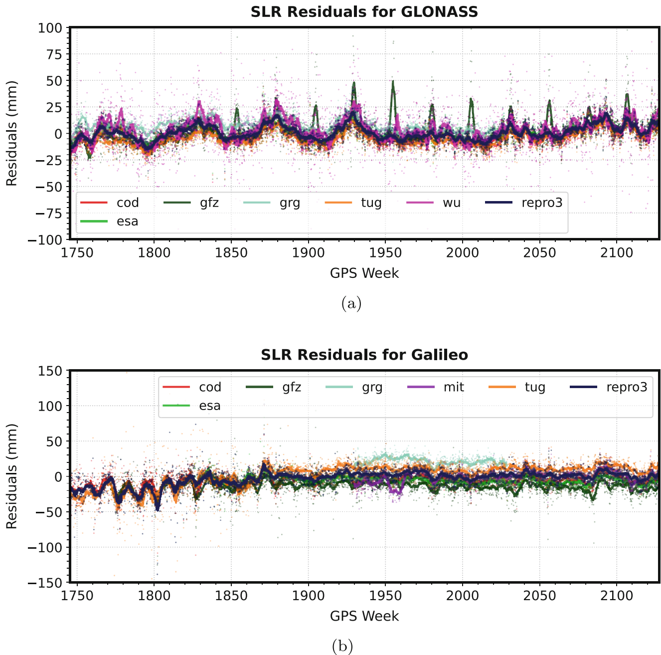
Fig. 3 Average SLR Residuals per constellation for each AC solution and the combination. (a) GLONASS. (b) Galileo
