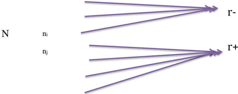
Fig. 3. Schema of the function R(N) that is not injective, i.e. which associate different values n_i \neq n_j to the same value of R .
