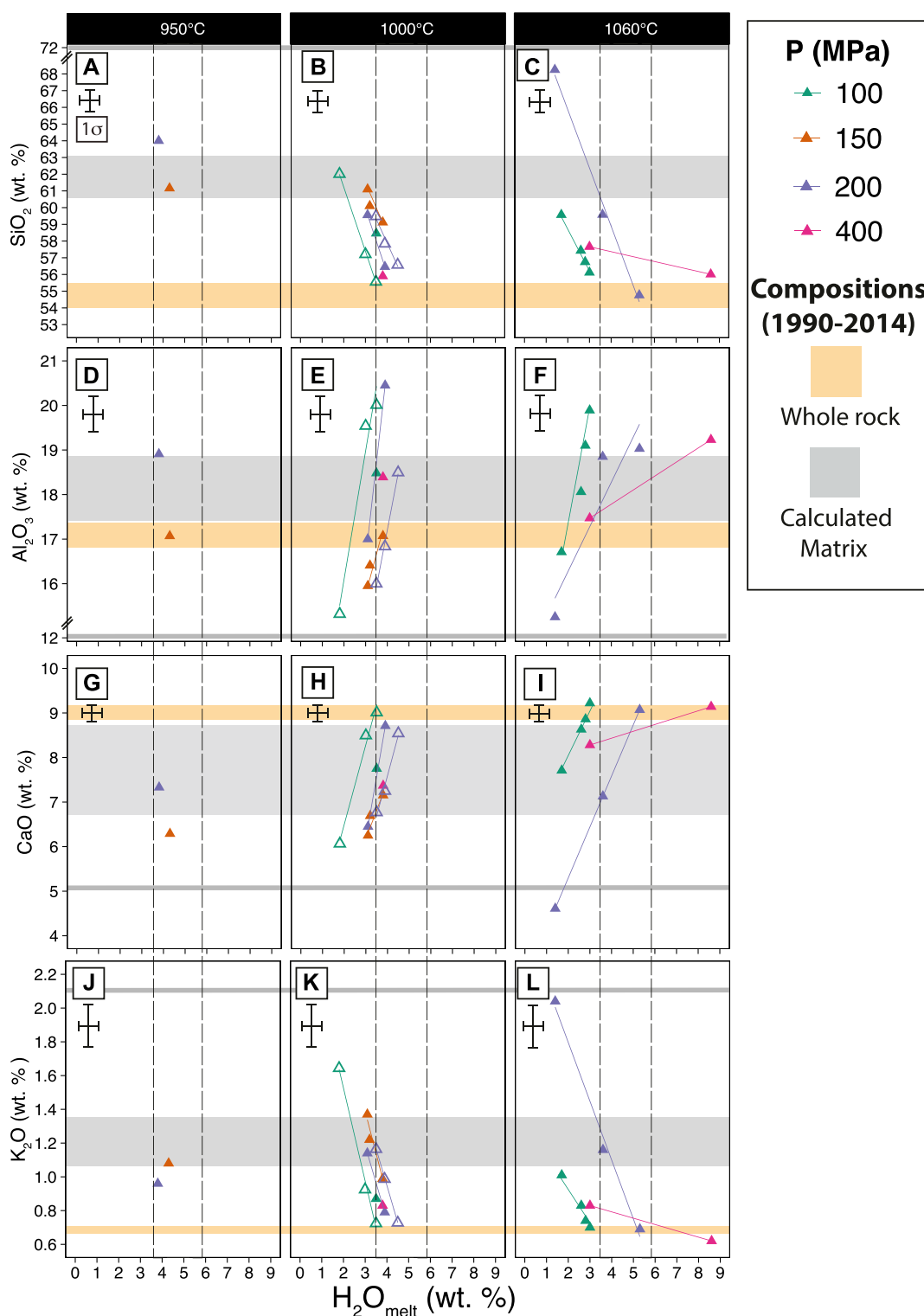
FIGURE 5 Major element oxide compositions of experimental glasses (in wt%) vs. dissolved water content in the melt according to three different temperatures SiO 2 (A) 950°C, (B) 1,000°C, (C) 1,060°C; Al 2 O 3 (D) 950°C; (E) 1,000°C, (F) 1,060°C; CaO (G) 950°C; (H) 1,000°C; (I) 1,060°C; K 2 O (J) 950°C, (K) 1,000°C, (L) 1,060°C. Yellow horizontal band denotes the range of whole rock compositions. The thick gray band is the composition of calculated matrix for the explosive eruptions (1990, 2014); the thin gray band is the calculated matrix of the 2007 dome (Table 1). The calculated matrix compositions for the 1990, 2007, and 2014 eruptions were estimated by mass balance calculations (Albarede, 1995) (see Methodology section). Vertical dashed lines are water content in the melt inferred from crystallinity and phase assemblage (Figures 3, 4). Filled symbols represent experiments at NNO; open lined symbols represent experiments at NNO +2.
