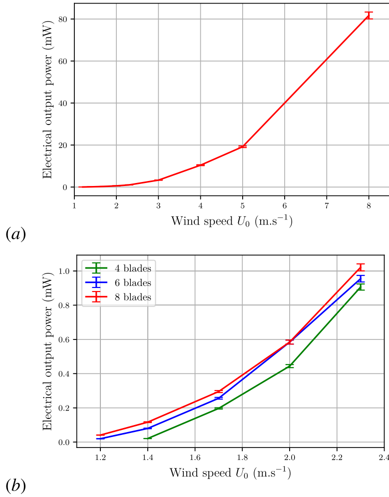
Fig. 12. Maximum output power (a) for each wind speed tested for the optimal propeller and (b) for wind speeds between 1.2 and 2.3 \text{m s}^{-1} for propellers with 4, 6 and 8 blades, \alpha_p = 30^\circ and \beta = 5^\circ .
