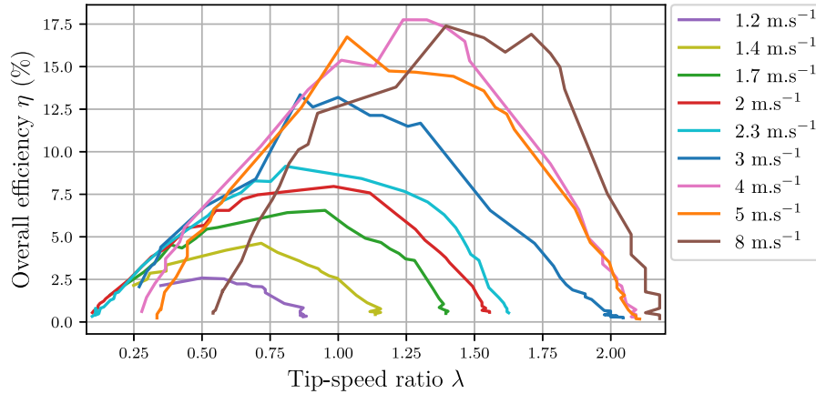
Fig. 13. Overall efficiency as a function of the tip-speed ratio for various wind speeds.
