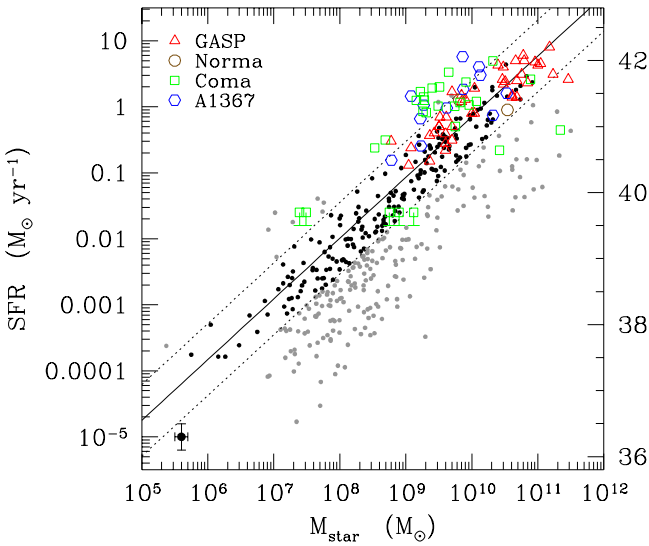
Fig. 7. Main-sequence relation for galaxies coded according to their distance to the best fit derived for HI gas-rich late-type systems. Filled black dots show galaxies within 1\sigma from the relation, and filled grey dots show galaxies >1\sigma above or below the relation. The solid line gives the best fit obtained for gas-rich star-forming systems, and the dotted lines show the limits 1\sigma above and below the best fit. Galaxies undergoing a ram-pressure-stripping event identified in Boselli et al. (2022a) are indicated with large empty coloured symbols: brown circles show those belonging to the Norma cluster, green squares stand for Coma, and blue hexagons represent A1367. Red triangles indicate the jellyfish sample of Vulcani et al. (2018) . Star formation rates and stellar masses are derived consistently with those measured within the Virgo cluster. The typical uncertainty on the data is shown in the lower left corner.
