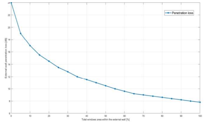
Figure 5: Penetration loss for different percentage of glass mounted in the external wall.
