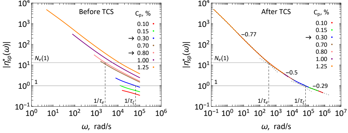
FIG. 9. (color online) Left: Micro-rheological absolute specific viscosity |\eta_{sp}^*(\omega)| for PEO aqueous solutions. Polymer concentration C_p is different for each curve. We obtain \tau_\xi = 0.000015 s for C_p = 0.3\% and \tau_e = 0.00038 s for C_p = 0.8\% . Right: Master curve of |\eta_{sp}^*(\omega)| constructed by shifting the original curves shown in the left panel. Reference polymer concentration is 0.3 %. We obtain \tau_e = 0.0028 s and \tau_\xi = 0.000015 s for this reference polymer concentration (0.3%). Probe concentration is 1%.
