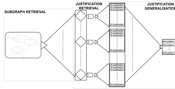
Fig. 3: Diagram that shows the pipeline used to extract subgraphs, find justifications in these subgraphs, and generalise these justifications to anti-patterns.
