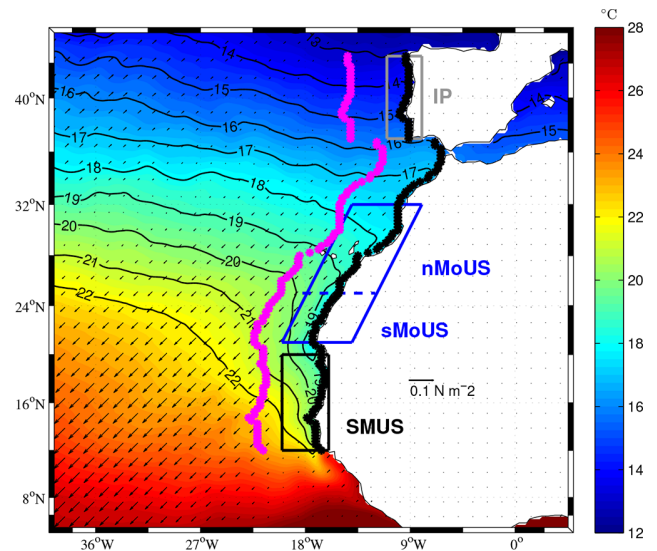
Figure 1. Colors: OISSTv2 climatological mean (°C) in March averaged over the 1992–2011 period. Black vectors show the wind stress from the Cross-Calibrated Multi-Platform (CCMP; computed offline from winds as described in the Appendix). The referent vector is shown inland, and the contours show some SST values. The gray box (37–43° N, 8–11° W) represents the Iberian Peninsula region (IP); the black box (12–20° N, 16–20° W) represents the Senegalo–Mauritanian subregion (SMUS). The inclined blue box outlines the Morocco (MoUS) subdomain (21–32° N), with a dashed blue line representing the northern boundary of the southern Morocco subdomain (sMoUS). The stars indicate the coastal (black) and offshore (magenta) locations used for the computation of the thermal upwelling index (see Sect. 2.3). The black and magenta dots are separated by 5° of longitude.
