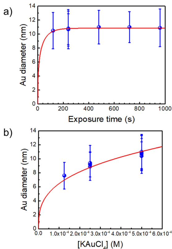
Fig. 1 (a) Au NDs growth versus exposure time for [\text{Au}^{3+}]_0 = 0.5 \text{ mM} (the red line is a fit according to dynamic modelling presented in Ref. 35. (b) Variation of the Au NDs size at completion vs. [\text{Au}^{3+}]_0 (the fit corresponds to mass conservation at completion, see text). [\text{TiO}_2] = 5.5 \text{ mM} and P = 56.1 \text{ mW} for all experiments.
