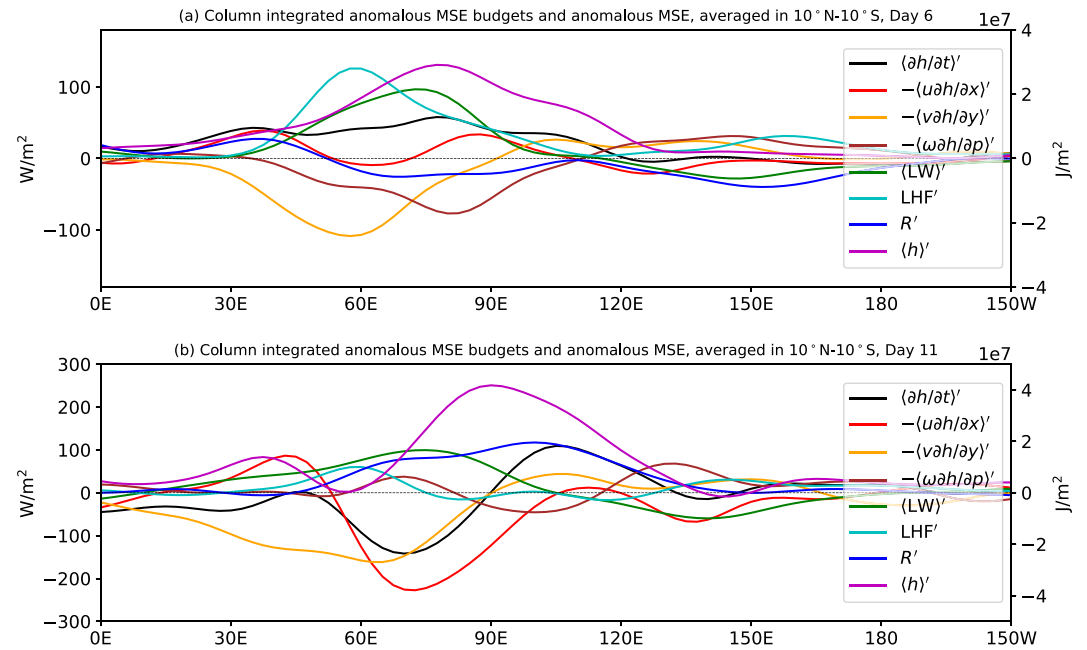
Figure 4. Anomalous moist static energy (MSE) budget terms in Equation 4 averaged between 10°N and 10°S, on (a) day 6 and (b) day 11, in units of W/m 2 . The anomalous shortwave heating term, \langle SW \rangle' , and the anomalous surface turbulent sensible heat flux term, \langle SHF \rangle' , are too small in comparison with the other terms and therefore not plotted. The right vertical axis indicates the computed values for the equatorially averaged anomalous column integrated MSE, \langle h \rangle' , shown in magenta.
