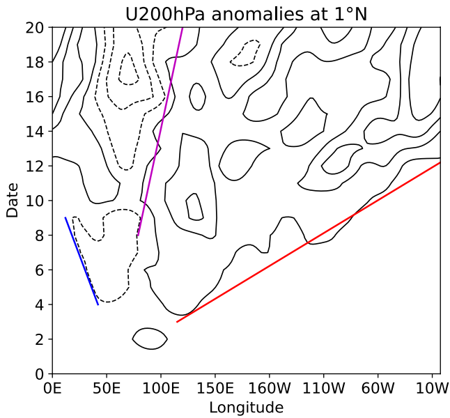
Figure 3. A Hovmöller diagram of zonal wind speed anomalies at 1°N, 200 hPa in the 3K perturbation experiment relative to the Control. The contour interval is 10 m/s, with solid and dashed contour lines starting at \pm 5 m/s, respectively. The eastward propagating Kelvin wave front is indicated by the red line, the westward propagating Rossby wave front by the blue line, and the excited Madden-Julian oscillation event by the magenta line.
