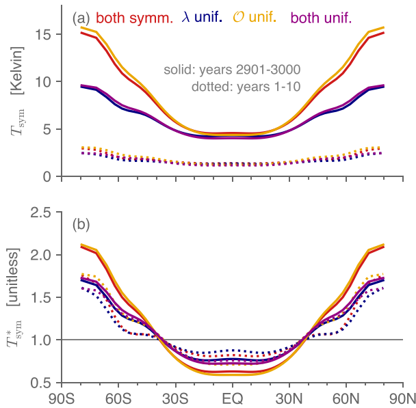
FIG. 6. Surface air temperature response in MEBM simulations corresponding to years 1–10 (dotted curves) and years 2901–3000 (solid curves) of the CESM1 4 \times \text{CO}_2 simulation, shown either (a) raw (in K) or (b) mean-normalized (unitless). Colors correspond to simulations with (red) both \lambda and \mathcal{O} symmetrized but not uniform, (blue) \lambda set to its global-mean value at all latitudes, (yellow) \mathcal{O} set to its global-mean value at all latitudes, or (purple) both \mathcal{O} and \lambda set to their global-mean values at all latitudes.
