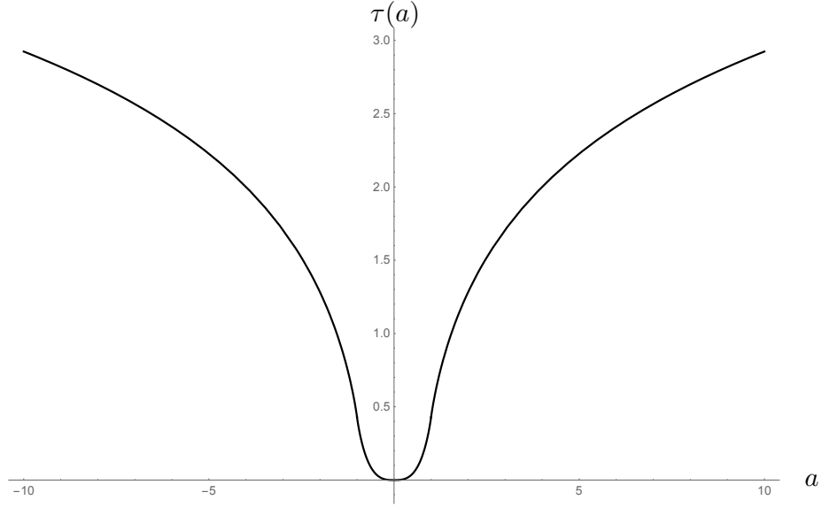
Figure 3: The dynamics across the singularity is regular due to inverse volume corrections. In this picture we show the function \tau(a) , defining the dynamical evolution across the singularity, in the case of Thiemann's regularization of the inverse-area-operator.
