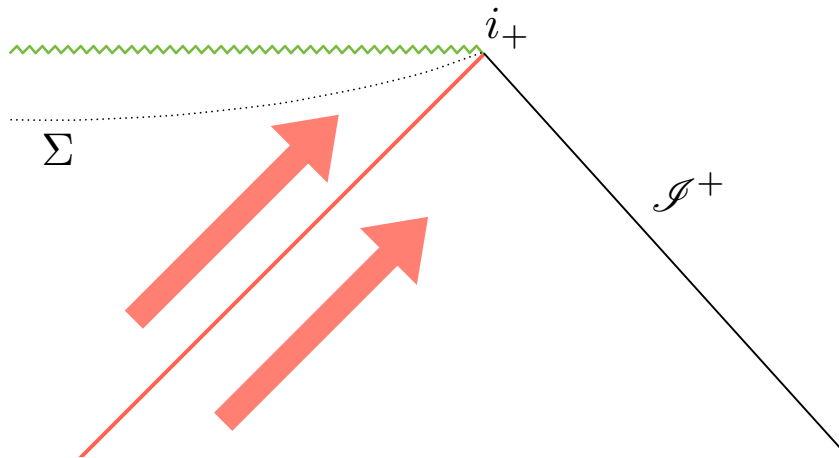
Figure 2: Hawking pairs produced in a black hole spacetime with M \gg m_p are described as test field excitations on a background spacetime that is idealized by a stationary black hole solution in the region of the Penrose diagram away from the collapsing matter and containing i_+ . Stationarity implies the existence of a conserved energy-momentum current used, in this paper, to relate the value of p_\phi in the KS model to the frequency of the emitted particle at \mathcal{I}^+ and (via Hawking temperature) to the black hole mass M .
