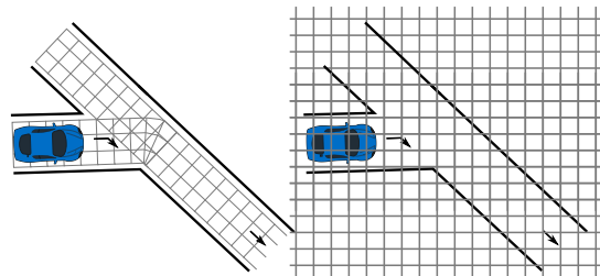
Fig. 4: Left: an LGM for a merging intersection. The ego vehicle (blue) intends to turn right. Right: A Cartesian OG.
