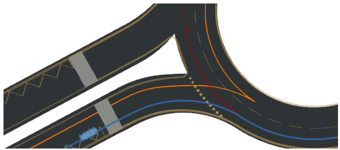
Fig. 3: Lanes of interest in a real experiment led in Compiègne. The ego vehicle is represented in blue and its intended path represented by the blue line. The red line represents lanes in direct interaction with the ego vehicle path and the orange lines are lanes that interact indirectly.
