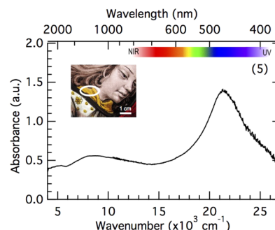
Figure 5. Optical absorption spectrum of the yellow staining on the collar of the angel (inset).
