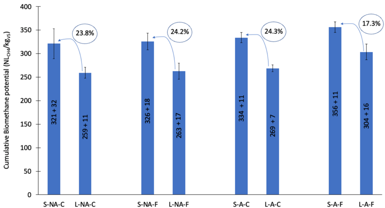
Figure 4. Total cumulative methane yield after 57 days.
