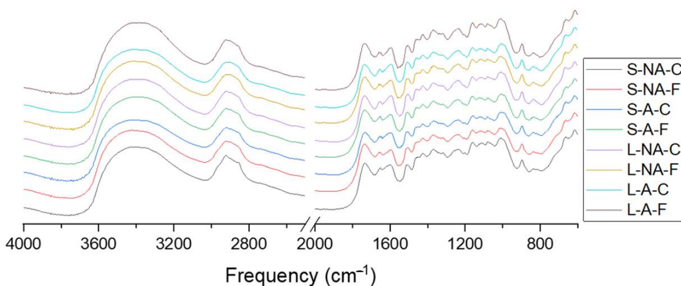
Figure 8. DRIFT spectra of control and pretreated samples.
