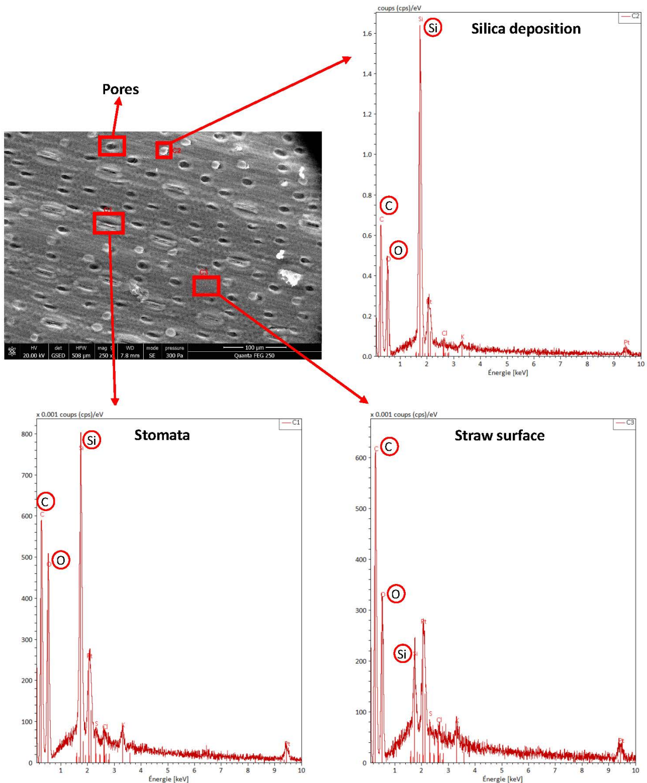
Figure 6. SEM-EDS analysis of the S-A-C straw sample.
