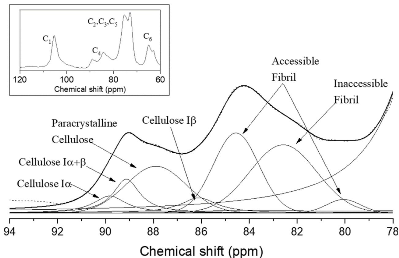
Figure 12. Fitting of the C_4 -region S-NA- straw sample). The dotted lines represent the experimental spectrum. The fitted lines and their superposition (ticker line) are shown as solid lines. In the inset on the top left, the NMR spectral region of S-NA-C with the cellulose peaks attribution [73].
