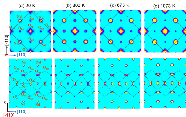
Fig. 6 Maximum entropy analysis of single crystal neutron diffraction data of \text{Nd}_2\text{NiO}_{4.23} obtained at (a) 20 K, (b) 300 K, (c) 673 K, and (d) 1073 K. (Upper row) (110) - (\bar{1}10) projection of 2D nuclear density maps particularly showing O_{\text{ap}} displacements toward the nearest O_{\text{int}} site. The black continuous line outlines the F -centred average chemical unit cell. (Lower row) (110)/(001) projection of 2D nuclear density maps displaying the O_{\text{ap}} - O_{\text{int}} - O_{\text{ap}} oxygen diffusion pathway along the [110] direction. Single crystal data at 20 K and 300 K were recorded on ZEBRA/TriCS ( \lambda = 1.178(1) \text{\AA} ) at SINQ, PSI while 673 K and 1073 K data were measured on D9 ( \lambda = 0.837(1) \text{\AA} ) at ILL.
