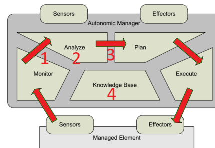
Fig. 1. The MAPE-K model
