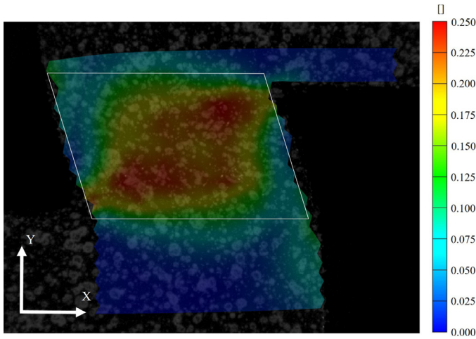
Fig. 7. Equivalent plastic strain field ( T = 600\text{ }^{\circ}\text{C} ).
