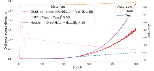
Figure 7: Colored MNIST dynamics with ERM.
