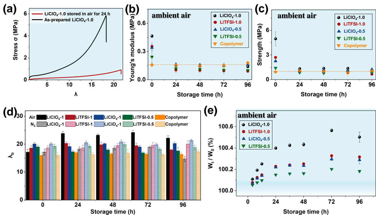
Figure 2. Mechanical properties and weight change of air-aged ICEs. (a) Representative stress-stretch curves of the as-prepared ICE ( \text{LiClO}_4\text{-1} ) and that aged in air for 24 h. (b), (c) Young's modulus and tensile strength of the ICEs and the pure copolymer during 96 h storage in ambient air. The values are measured at 24 h intervals. (d) Stretch at break \lambda_b of ICEs and the pure copolymer stored in air or nitrogen environments. (e) The weight change of the air-aged ICEs due to water absorption when stored in ambient air. Five samples are tested for each data point.
