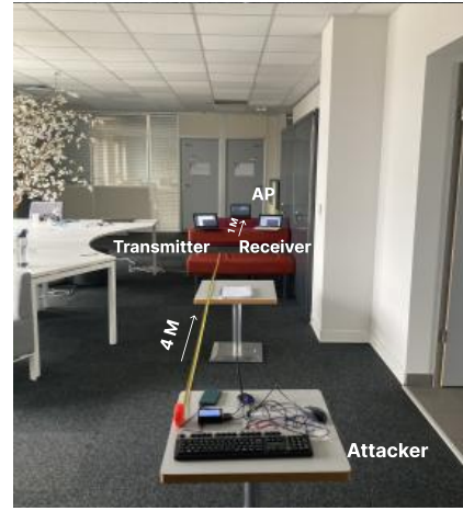
Fig. 2: Testbed implementation
