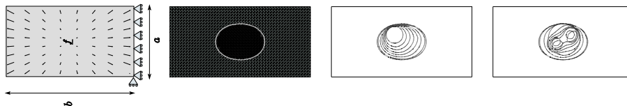
Figure 1: Application of the method on a simple case. From left to right, mechanical setting, mesh and constrained zone for both methods, evolution of the constrained zone during the iteration for two different starting configuration using the new method.
