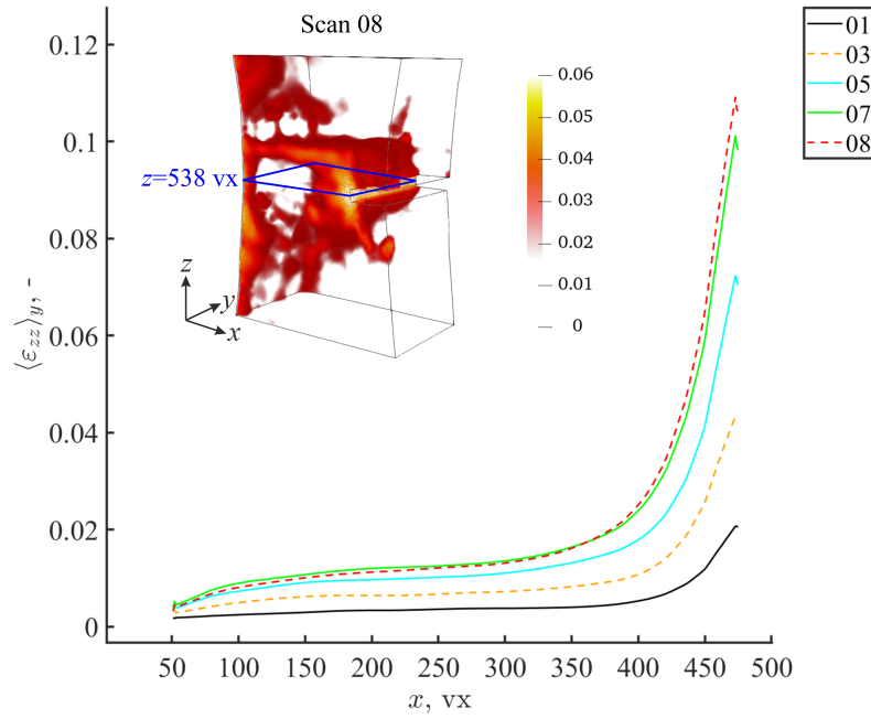
Figure 5. \varepsilon_{zz} strains averaged through the material thickness ( y -direction) and extracted for the mid-height notch plane ( z = 538 vx). The averaged \varepsilon_{zz} strains were computed for the scans acquired at the peak of the prescribed loading cycles ( i.e. , scans 01, 03, 05, 07 and 08). The blue rectangle in the thresholded \varepsilon_{zz} field of scan 08 depicts the plane in which the through-thickness averaged \varepsilon_{zz} strains were assessed.
