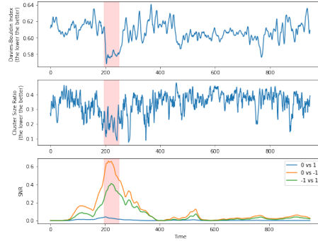
Fig. 3: Non-profiled leakage assessment, with area of interest (in red), performed on the collection of EM peaks of all the targeted coefficients. Top: DBI (the lower, the better). Middle: CSR (the lower, the better). Bottom: SNR with true labels (can only be performed when knowing the keys).
