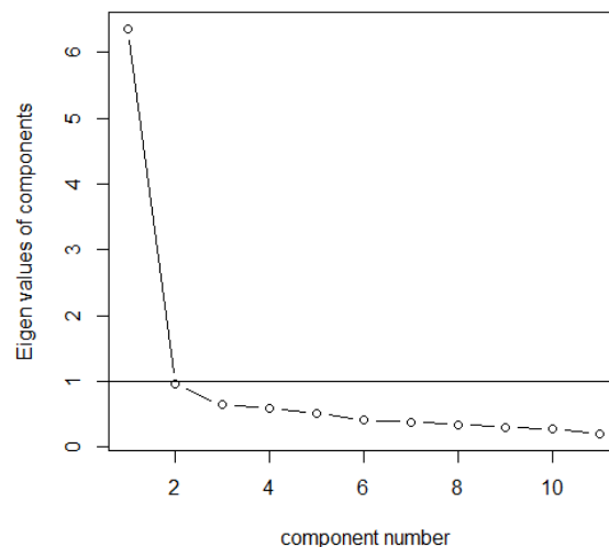
Figure 5. Scree plot
