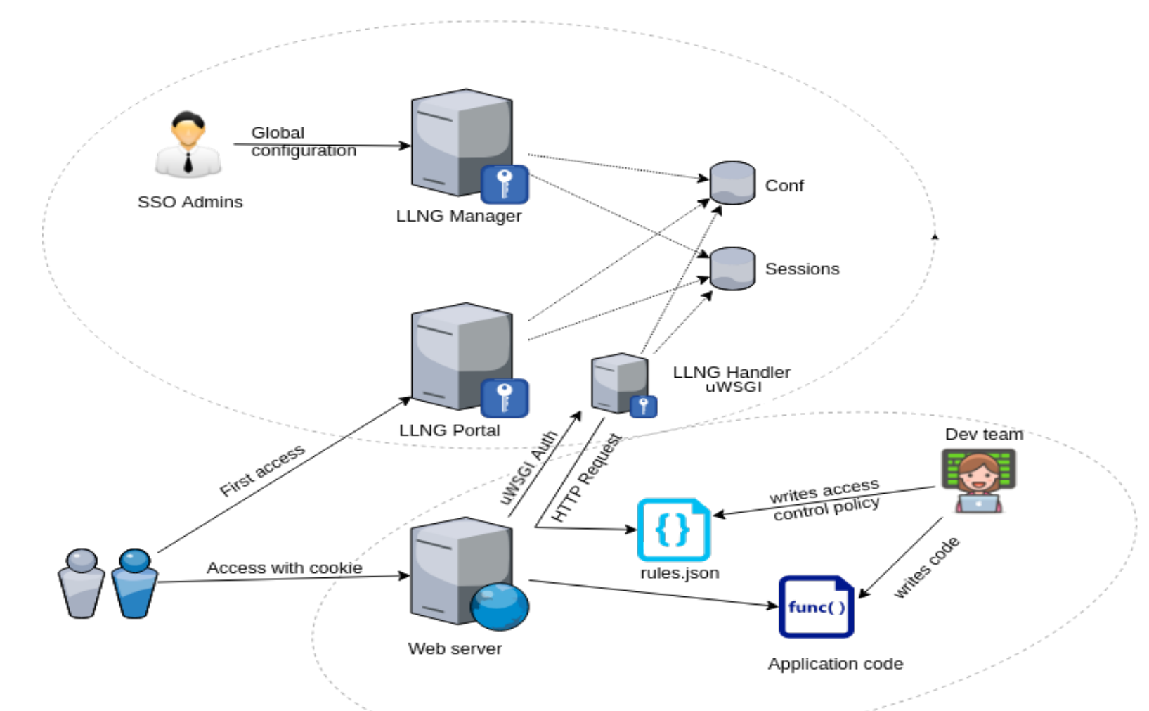
Figure 7: DevOps handler
