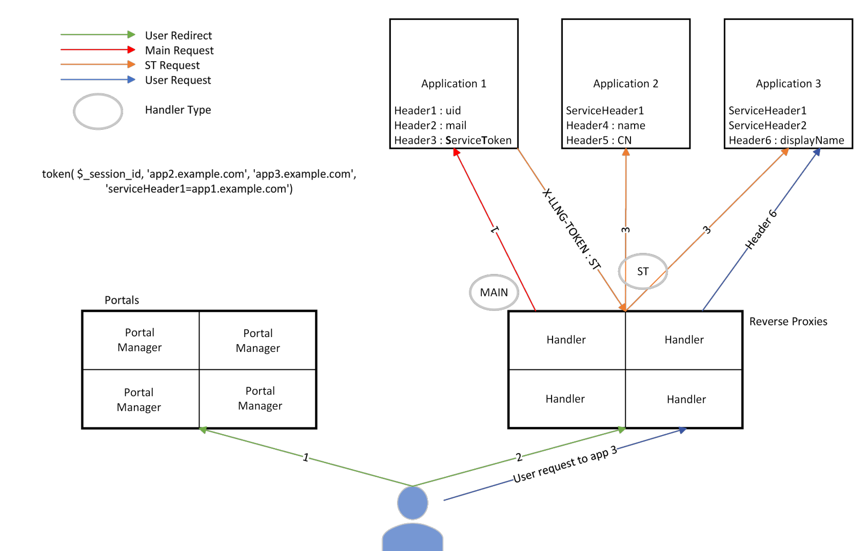
Figure 6: ServiceToken handler
