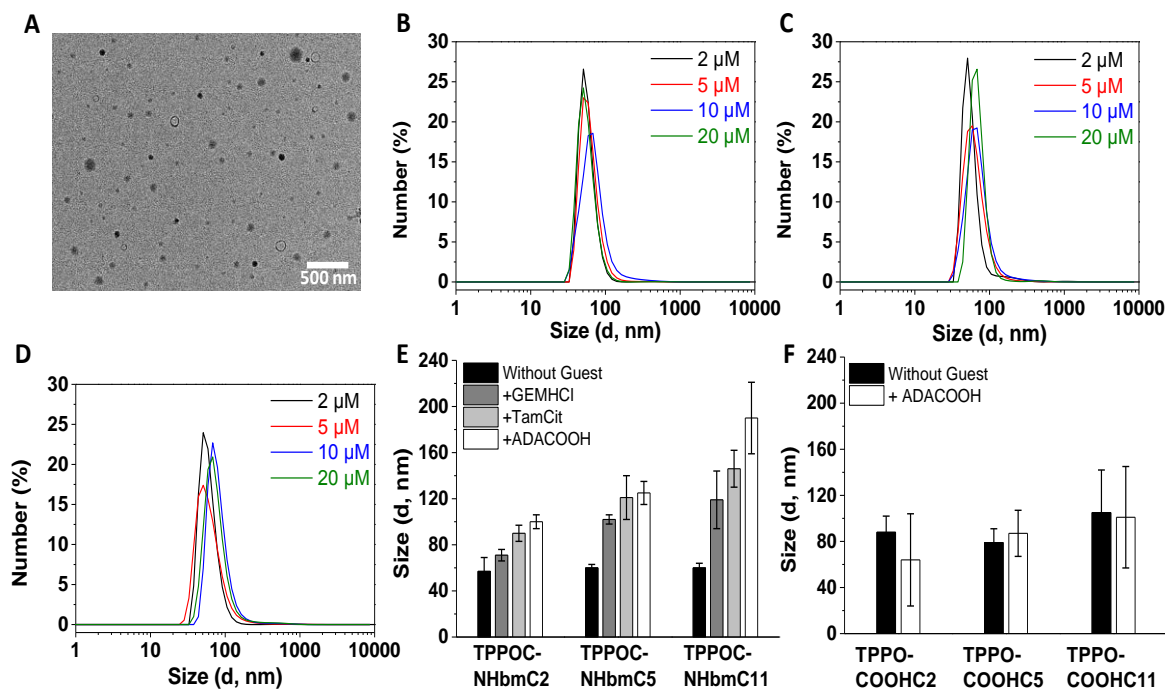
200 Fig. 2. (A) TEM image of TPPOCNHbmC11 NPs at 20 \mu\text{M} (without contrasting agent); (B-D) Number (%) vs size DLS profiles of (B) TPPOCNHbmC2 , (C) TPPOCNHbmC5 and (D) TPPOCNHbmC11 NPs at 2, 5, 10 and 20 \mu\text{M} concentrations in PBS*. DLS profiles of number (%) vs size of (E) TPPOCNHbmCx in comparison with (F) TPPOCOOHCx (2 \mu\text{M} in PBS) and in the presence of guest molecules ( GEM.HCl , TamCit , ADACOOH ). *PBS is with 4% DMSO (v/v), pH 7.4
