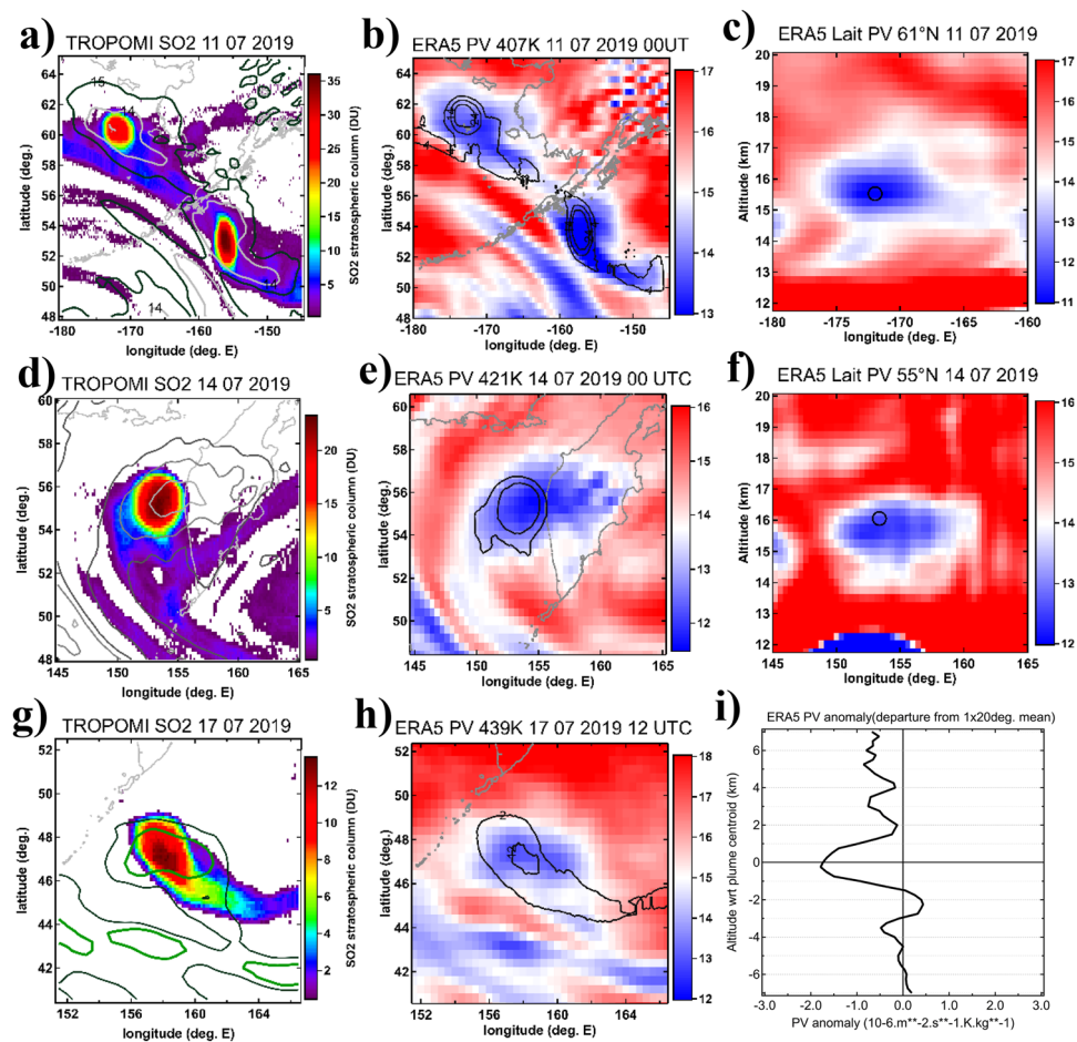
Figure 6. Potential vorticity of the vortex. (Left panels— a,d,g ) TROPOMI maps revealing isolated compact SO2 structure associated with the vortex on three different dates in July 2019. Contours indicate the corresponding low potential vorticity anomaly. (Middle panels— b,e,h ) ERA5 potential vorticity (PV in PVU, 1 \text{ PVU} = 10^{-6} \text{ Km}^2 \text{ kg}^{-1} \text{ s}^{-1} ) interpolated to the potential temperature level of the aerosol plume centroid derived from satellite observations. Black contours mark the corresponding SO2 plume displayed in the left panels. (Right panels— c,f ) Longitude-altitude sections of ERA5 Lait PV at the latitude of the primary VVP. The black circle marks the corresponding aerosol plume location derived from satellite observations. ( i ) Composited PV anomaly altitude profile with respect to the aerosol plume centroid obtained from ERA5 data between 25 July and 10 August. The PV anomaly is obtained as a deviation from an average PV profile within 1^\circ latitude \times 20^\circ longitude bin.
