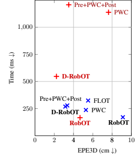
Figure 4: Evaluation on the Kitti dataset for 3D scene flow. Black numbers and crosses (×) correspond to results on scene pairs that are sampled with 8,192 points per frame; red numbers and plus signs (+) correspond to scene pairs that are sampled with 30,000 points per frame.
