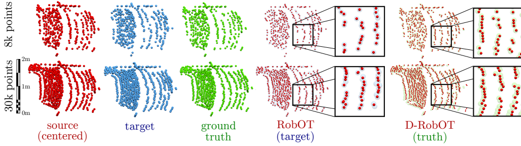
Figure 3: Influence of the sampling density on a detail (top car) of the Kitti frames of Fig. 1.b. First row: On sub-sampled 3D scenes, the regularizing priors of the D-RobOT architecture prevent over-fitting to the random sampling patterns of the target point cloud (blue). The D-RobOT output (last column, red) is very close to the ground truth scene flow (green). Second row: Increasing the number of points per frame reduces the influence of sampling artifacts. The simple RobOT baseline (fourth column, red) still over-fits to the target (blue) but becomes remarkably competitive.
