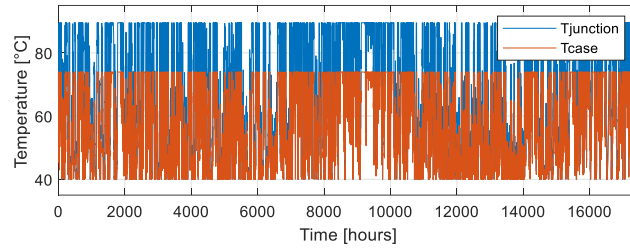
Fig. 3: Thermal profile of T2 under the evaluated period for the studied mission profile
