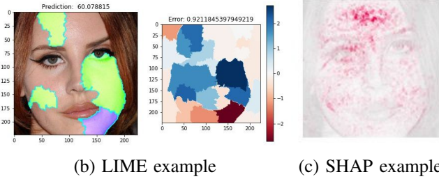
Fig. 2. Explainability approaches applied to the VIP_attribute dataset.
