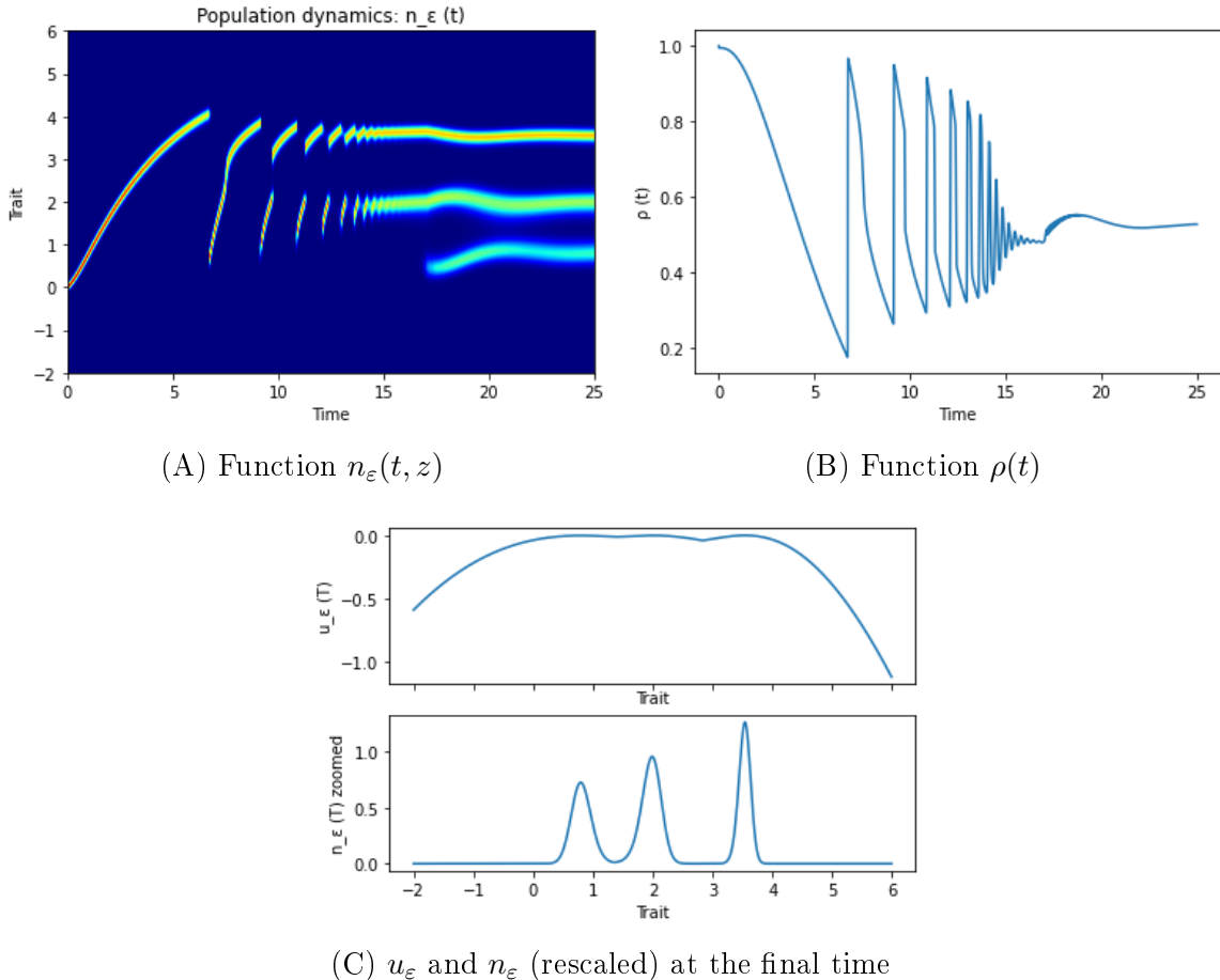
Figure 3: Solution of (17) in the trimorphic case \mu = 5 , with values \tau = 0.5 , g = 0.05 and \varepsilon = 5 \cdot 10^{-4} .
