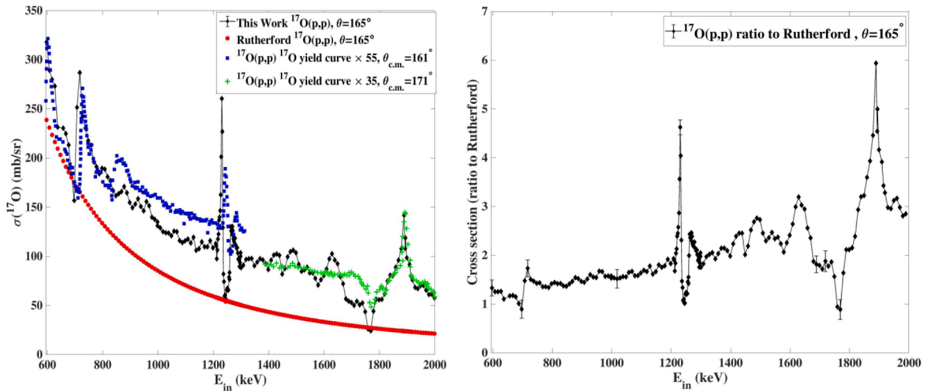
Fig. 9. a) Our measured proton elastic scattering cross-section, compared with scaled yield curves from Ref. [8,9]. b) The ratio to the Rutherford cross section of ^{17}\text{O} at 165^\circ for E_p = 0.6\text{--}2 MeV in the laboratory system. The representative uncertainty bars in b) represent the statistical uncertainty.
