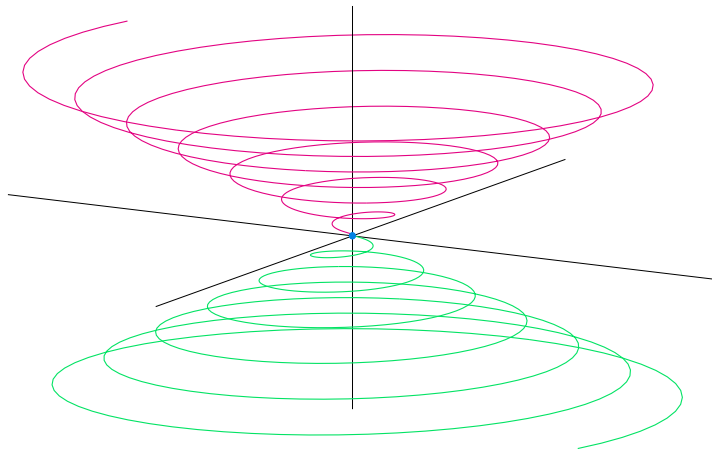
FIGURE 3. Graphic simplification of a Cartanian non-3D—or non-(1 + 3)D—space-time with double spiraling torsion. Try to visualize, imaginatively, an action à la Petti–Popławski [94] [102] of a #E30382-black hole, on one side, and of a #03E364-white hole, on the other
