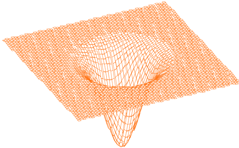
FIGURE 2. Semi-destruction of a non-3D—or non-(1+3)D—spatio-temporal #FF7518-grid with increasing gravitational field strength. Exactly like in the Fig. 1, here is a crude representation along the z -axis. Actually, when the gravitational force becomes infinite ( façon de parler ), is mandatory to switch to an unknown tiling, whether periodic or aperiodic, as a covering of the plane; we must correspondingly return to a Flatland-like scenario
