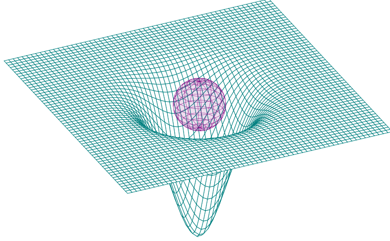
FIGURE 1. Curved space-time in a #008080-grid within the framework of a (pseudo-)Riemannian geometry, along the z -axis: we are looking at something like a non-3D space-time curvature, or non-(1 + 3)D space-time curvature, to be picky. The massive central body is #800080-colored
